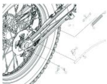
Homologation Kit
